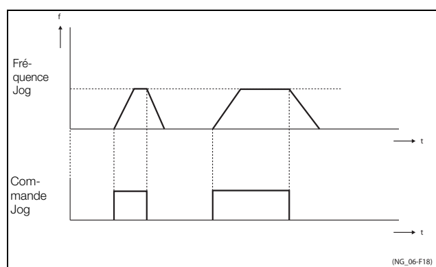
Fig. 105 Commande Jog
