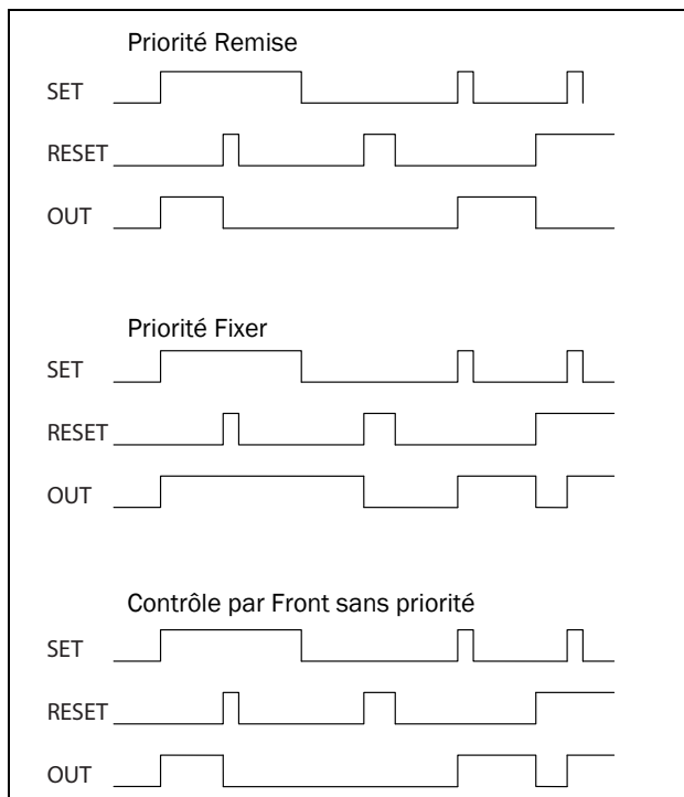
Fig. 140 Modes Flip-flop programmables.
